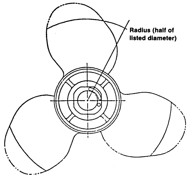
Modified Propeller
