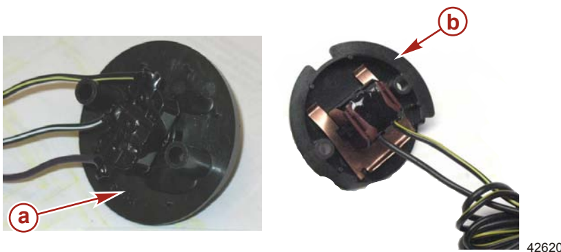
Old vs. new lanyard a - 87-19674Q2 b - New style
