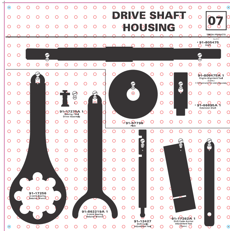
Board 7 (included in 8M0085504 and 8M0085505)
