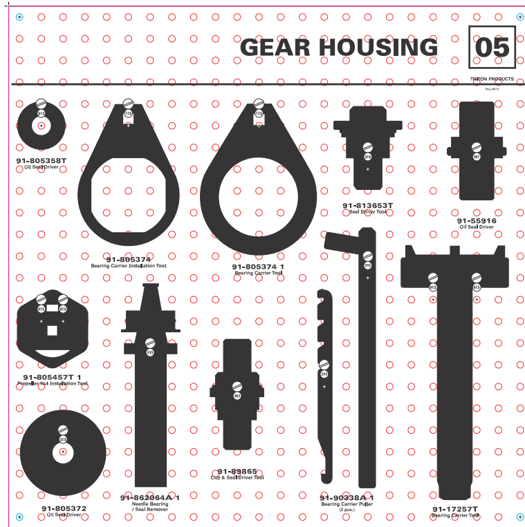
Board 5 (included in 8M0085504 and 8M0085505)
