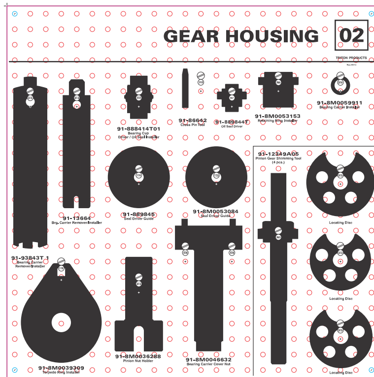
Board 2 (included in 8M0085503 and 8M0085505)
