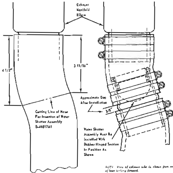
Figure 2. Exhaust Water Shutter Kit Installed
