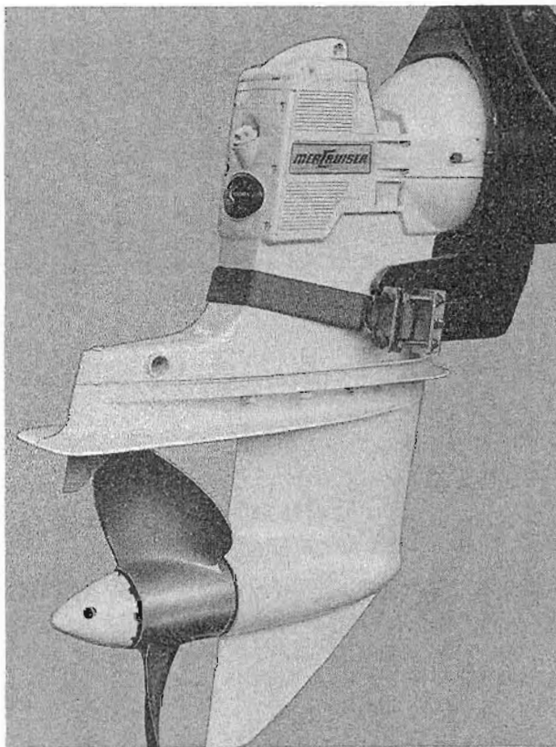
Figure 1. Tilt-Up Restraining Kit Installed on MerCruiser II
